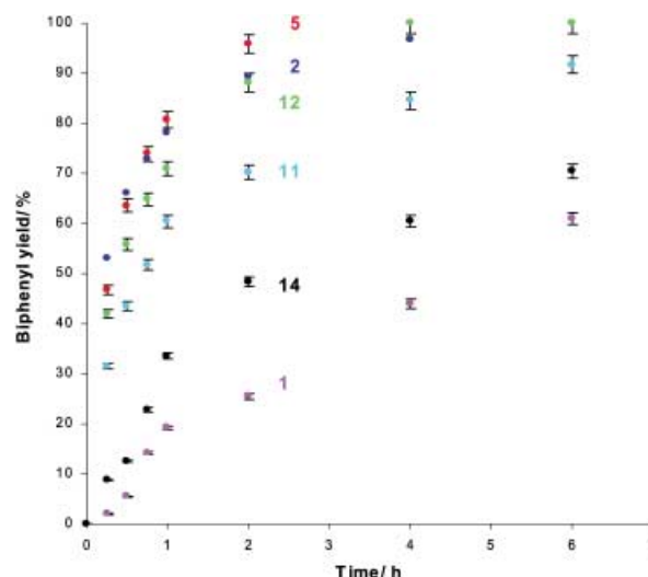
Figure 4. Time-resolved reaction profiles observed for Suzuki coupling of PhB(OH) 2 and PhI using various nanocluster catalysts. Duplicate experiments with catalysts 2 , 5 , and 12 were within \pm 3\% . Reaction conditions are as in Table 1.
