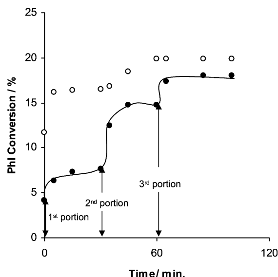
Figure 2. Suzuki coupling of PhB(OH) 2 with PhI catalysed by palladium nanoclusters (prepared via NaBH 4 reduction). Reaction conditions: 3.00 mmol PhI, 6.00 mmol PhB(OH) 2 , 6.00 mmol K 2 CO 3 , 50 mL toluene, 110 °C. (○) 1 mol % catalyst, added in one portion at t = 0; (●) 1 mol % catalyst in total, added in three equal portions at intervals of 30 min.
