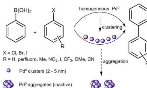
Figure 1. Cross-coupling of phenylboronic acid and halobenzene to give a biaryl derivative, showing clustering of the homogeneous palladium(0) catalysts followed by catalyst deactivation through aggregation.
