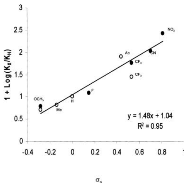
Figure 6. Plot of the relative rate constants vs. \sigma_p (Hammett plot); (○) results for cluster catalysts; (●) results reported for palladacycle catalyst in ref.[41]
