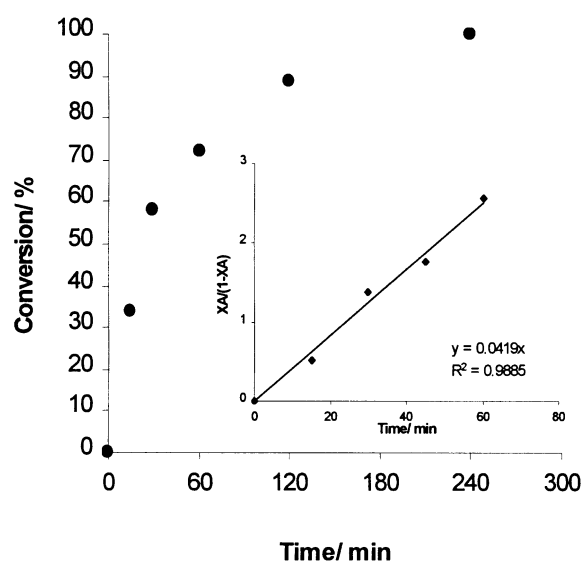
Figure 5. Suzuki coupling of PhB(OH) 2 with 4-bromobenzotrifluoride using a mixed Cu/Pd nanocluster catalyst. Inset shows the fit of the initial reaction rate to a second-order rate equation. Reaction conditions are as in Table 1.
